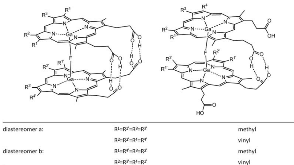
Figure 14. Proposed orientation of hydrogen bonding within a \mu -fluoro-bridged dimer of Ga(PPIX) based on NMR coupling evidence. All would coexist in a dynamic exchanging system.
